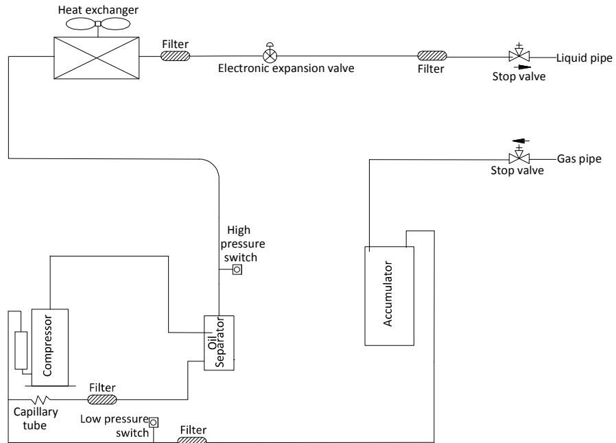
Figure 2-4.1: 30/40/50 model piping diagram
