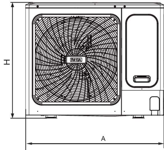
Figure 2-2.3: 60/70 model front view dimensions
