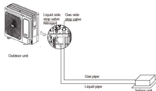
Figure 3-4.11: Gastightness test
