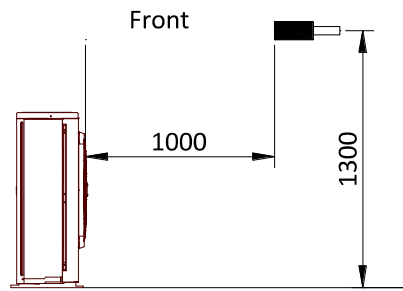
Figure 2-10.1: Sound pressure level measurement (unit: mm)
