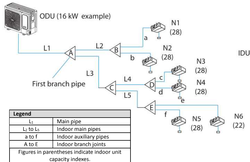
Figure 3-3.5: Refrigerant piping selection example
