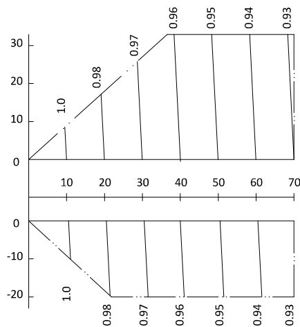
Figure 2-8.2: BCSF060, 070 rate of change in cooling capacity
