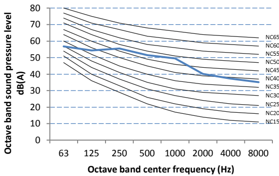
Figure 2-10.4 BCSF060N0A8-DTM160 octave band level
