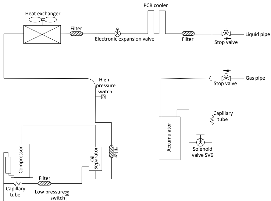
Figure 2-4.2: 60/70 model piping diagram
