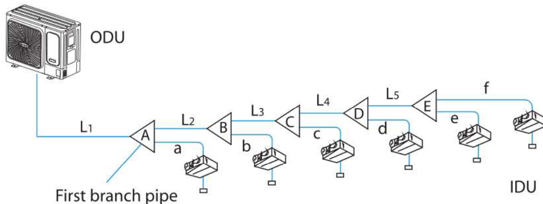
Figure 3-3.4: Selecting piping diameters
