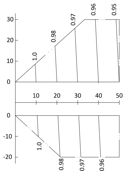
Figure 2-8.1: BCSF030, 040, 050 rate of change in cooling capacity
