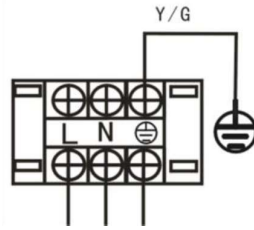
Figure 3-8.2: Outdoor unit 1-phase power supply terminals
