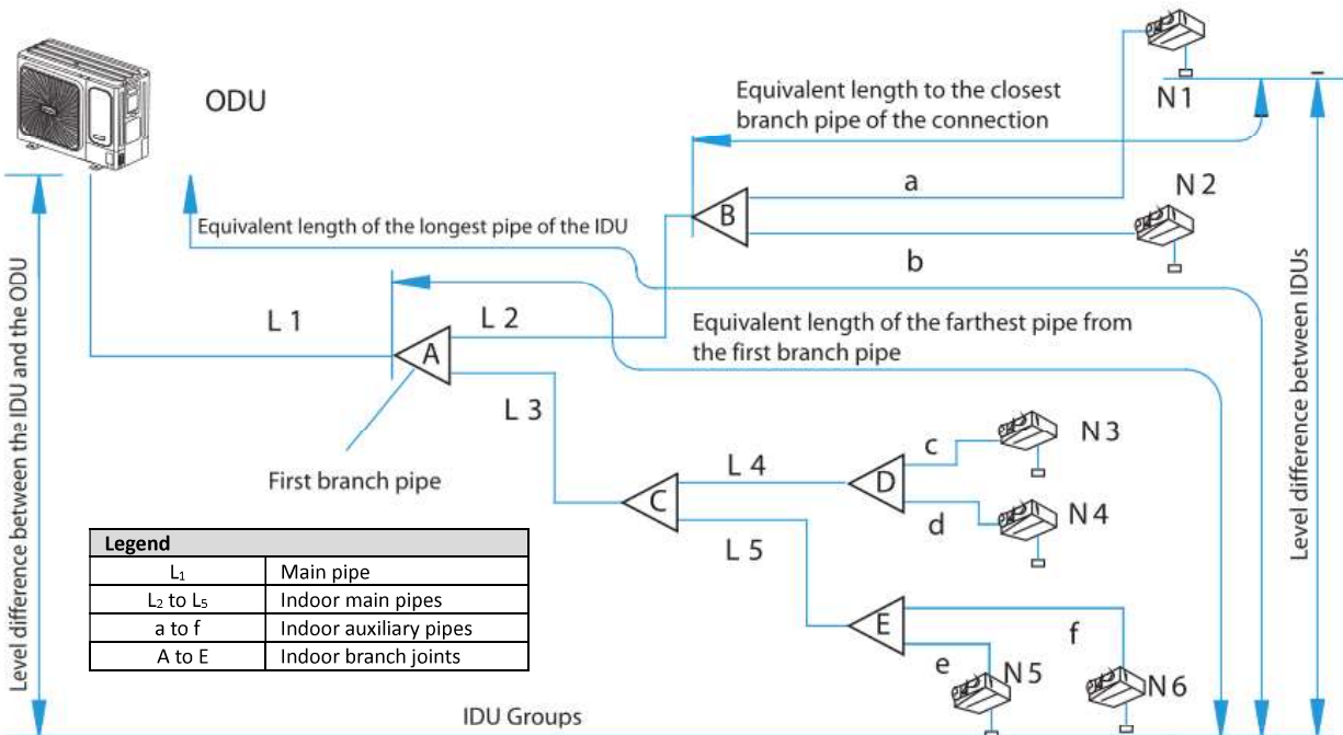
Figure 3-3.2: The second connecting method (Welding)
