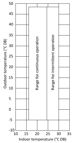
Figure 2-9.1: Cooling operating limits
