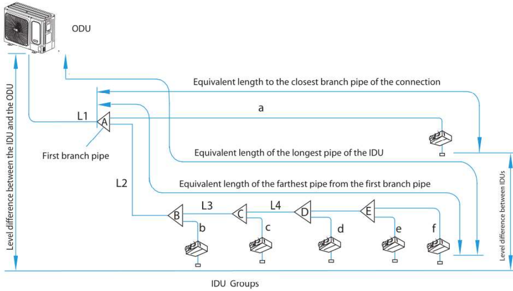
Figure 3-3.1: The first connecting method (Welding)
