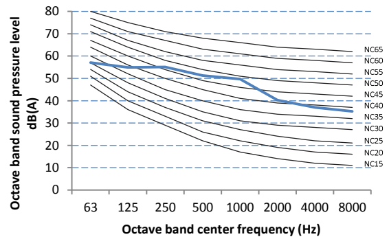
Figure 2-10.5 BCSF070N0A9-DTM190 octave band level
