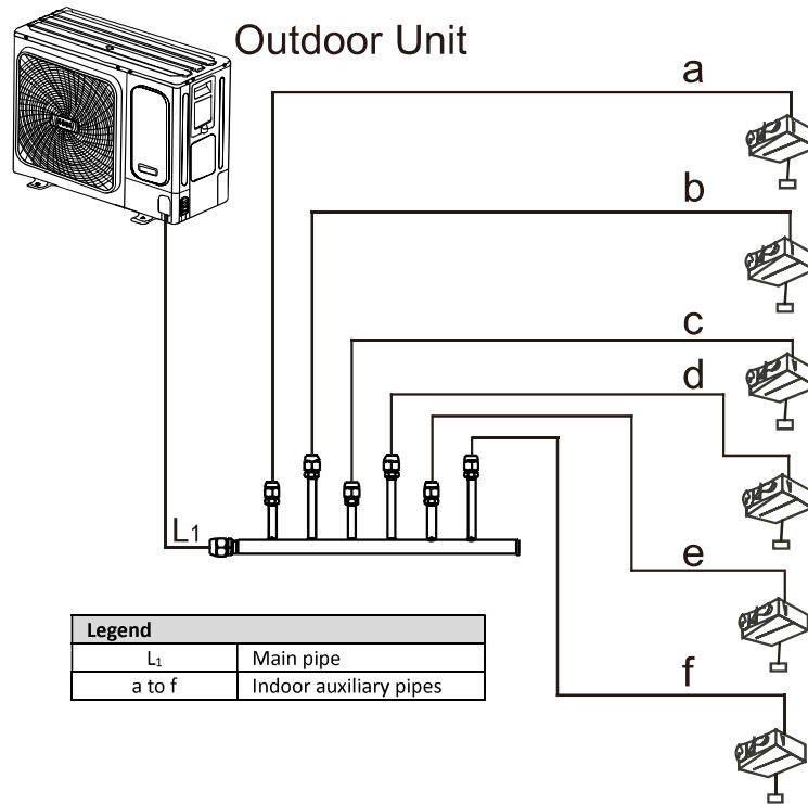
Figure 3-3.3: The third connecting method (Flaring)
